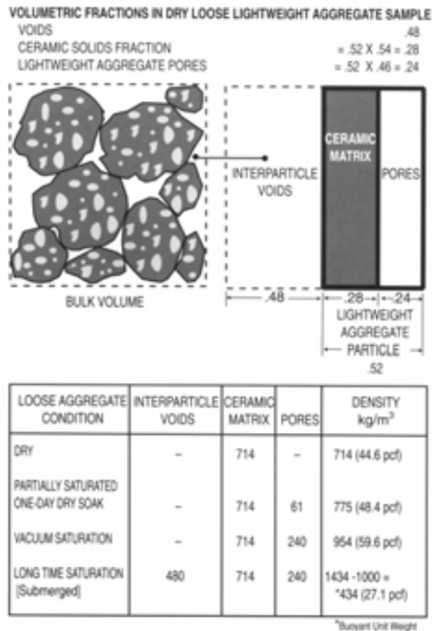
FIGURE 3 Voids, pores, and ceramic matrix fraction in a lightweight aggregate (LWA) sample
