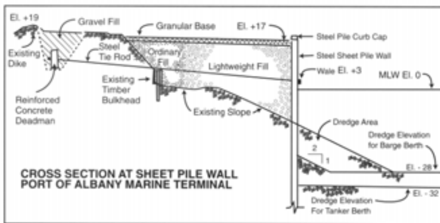
FIGURE 6 Rehabilitation of Port of Albany, New York 11981
