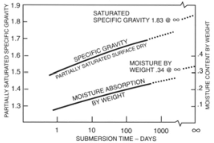
FIGURE 5 Moisture absorption (by weight) and partially saturated, surface dry specific gravity of lightweight aggregate (LWA) versus time of submersion absorption characteristics are shown in Figure 5 for a LWA sample with a measured 1-day immersion moisture content of 8.5% associated with a partially saturated surface-dry specific gravity of 1.5. When moisture absorption-versus-time relationships are extrapolated or theoretical calculations used to estimate the total filling of all the LWA pores, it can be shown that for this particular LWA the absorbed moisture content at infinity will approach 34% by weight with a totally saturated specific gravity of 1.83. Complete filling of all pores in a structural grade LWA is unlikely because the non-interconnected pores are enveloped by a very dense ceramic matrix. However, these calculations do reveal a conservative upper limit for submerged design considerations. Durability Characteristics
